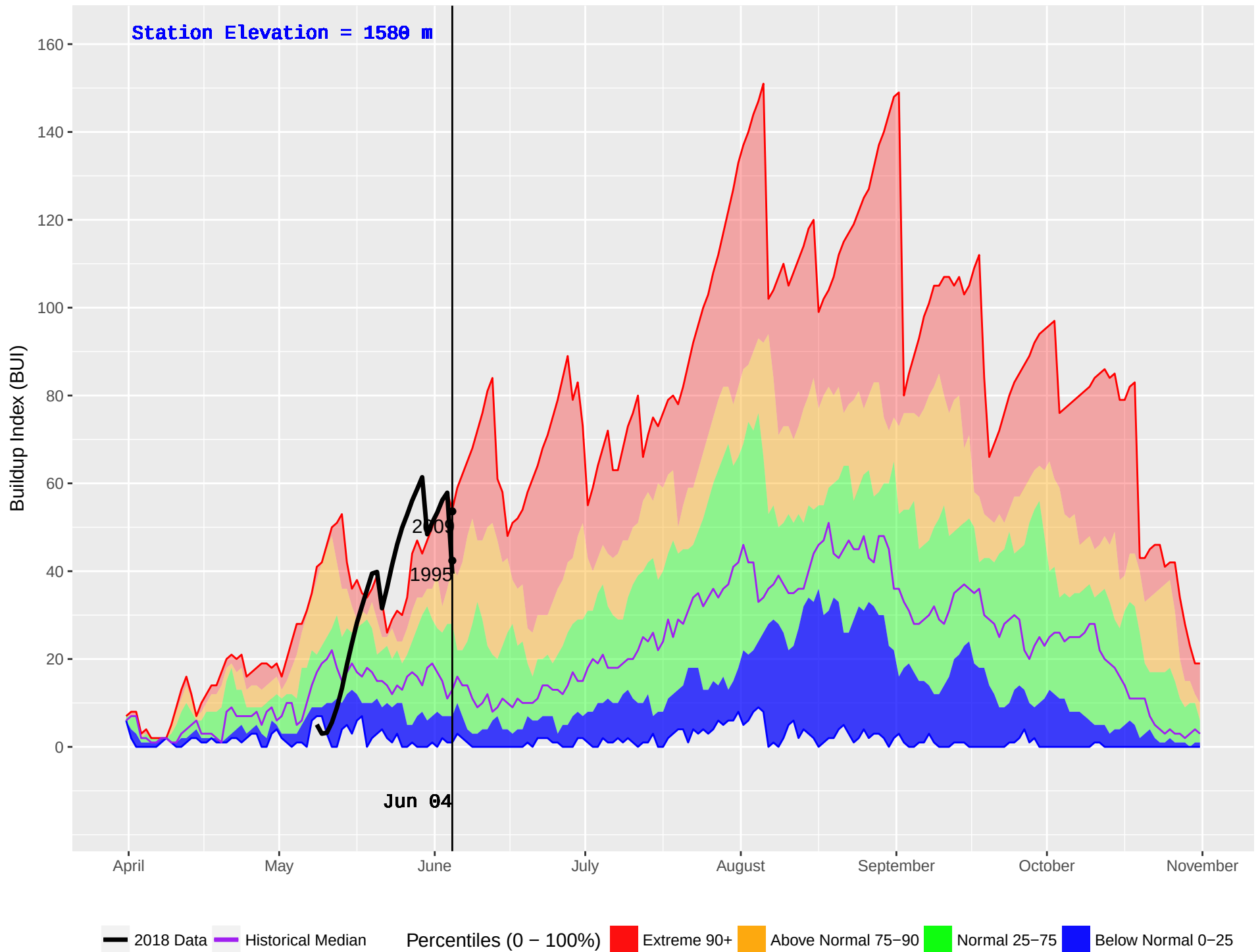
WINDY MOUNTAIN (244) : Historical (1989–2016) and Current (2018) Noon Buildup Index (BUI)
