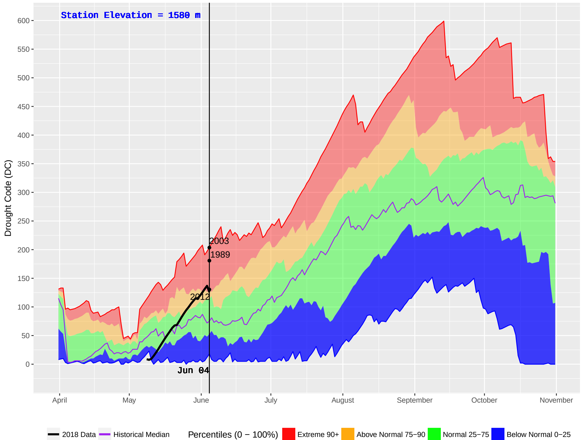
WINDY MOUNTAIN (244) : Historical (1989–2016) and Current (2018) Noon Drought Code (DC)
