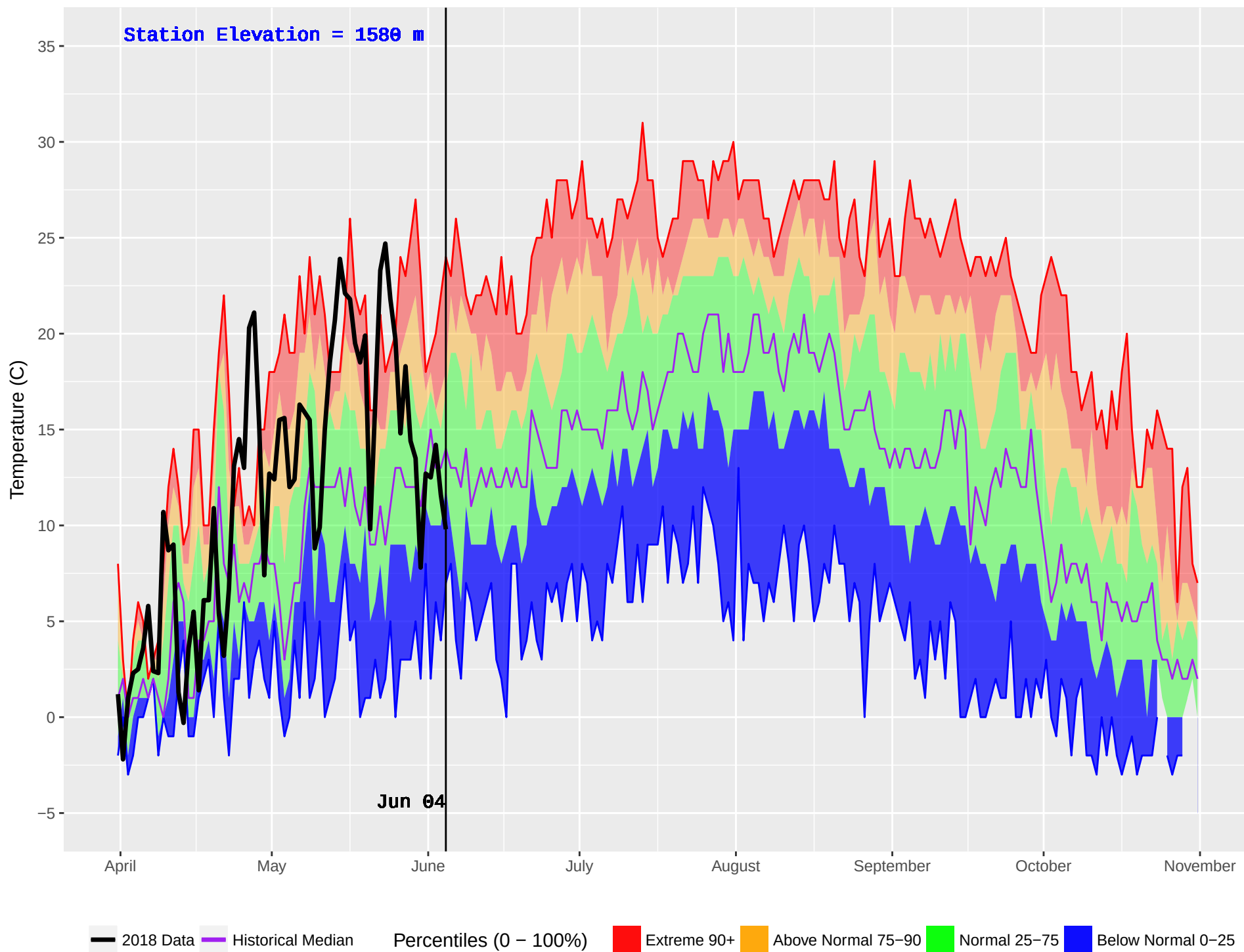
WINDY MOUNTAIN (244) : Historical (1989–2016) and Current (2018) Noon Temperature
